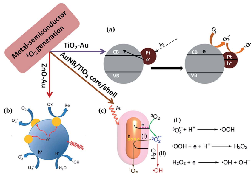
Fig. 11 Scheme illustrations of the proposed mechanism for plasmon-enhanced {}^1\text{O}_2 generation. (a) Au nanoparticle decorated on TiO 2 for {}^1\text{O}_2 generation, in which Au NPs enhanced the visible light photocatalytic efficiency by hot electron injection mechanism (b) proposed reaction mechanism for enhancement of {}^1\text{O}_2 generation using ZnO–Au NP hybrid catalysts. Deposition of Au onto ZnO increases the charge carrier separation and transport efficiency in photoexcited ZnO nanoparticles. (c) Generation of singlet oxygen ( {}^1\text{O}_2 ) through path (I) and hydroxyl radical \cdot\text{OH} through path (II) by using Au NR/TiO 2 core–shell nanostructure catalyst. Figures (a), (b) and (c) reproduced with permission from ref. 109, 111 and 112, respectively.
