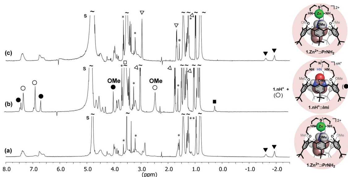
Fig. 4 ^1\text{H} NMR spectra (600 MHz, 298 K, DPC- d_{38} 20 mM in \text{D}_2\text{O} ) of (a) complex 1\cdot\text{Zn}^{2+} in the presence of \sim 4.5 equiv. of \text{PrNH}_2 and \sim 4 equiv. of Imi (pH = 10.5); (b) after the subsequent addition of DCl and \sim 106 equiv. of Imi (pH = 3.1); (c) after the subsequent addition of NaOD (pH = 8.8). \blacktriangledown : \text{PrNH}_2 in; \nabla : \text{PrNH}_2 out; \blacksquare : Imi in; \square : Imi out; \bullet : 1\cdot n\text{H}^+ ; \circ : 1\cdot n\text{H}^+ ; s: solvent.
