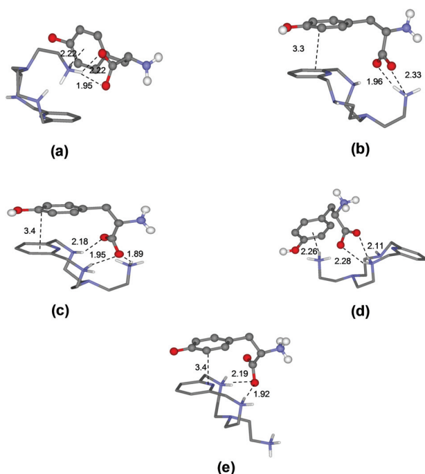
Fig. 3 Minimum energy structures calculated for the complexes [\text{HL1}-(\text{Tyr})]^{-} (a), [\text{HL1}(\text{HTyr})] (b), [\text{H}_2\text{L}_1(\text{HTyr})]^{+} (c), [\text{H}_2\text{L}_1(\text{H}_2\text{Tyr})]^{2+} (d), and [\text{H}_3\text{L}_1(\text{H}_2\text{Tyr})]^{3+} (e).
