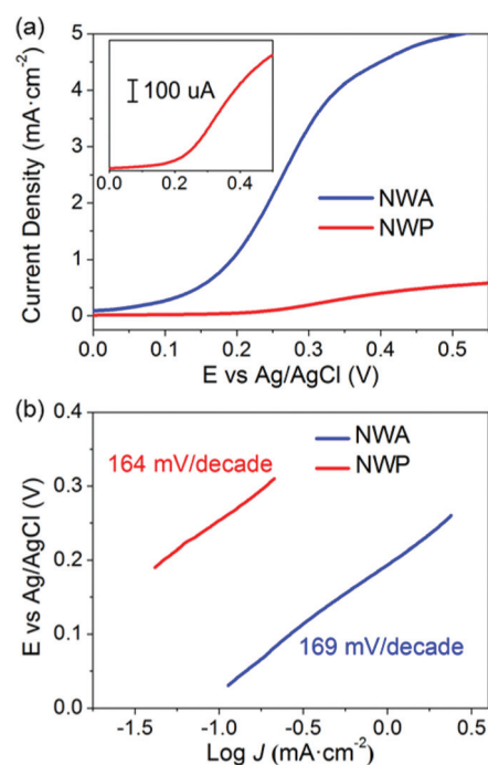
Fig. 5 (a) Positive scanning of CV measurements in the presence of 1 \text{ mM} glucose; inset shows the magnified curve for the NWP. (b) The corresponding Tafel plot of (a).
