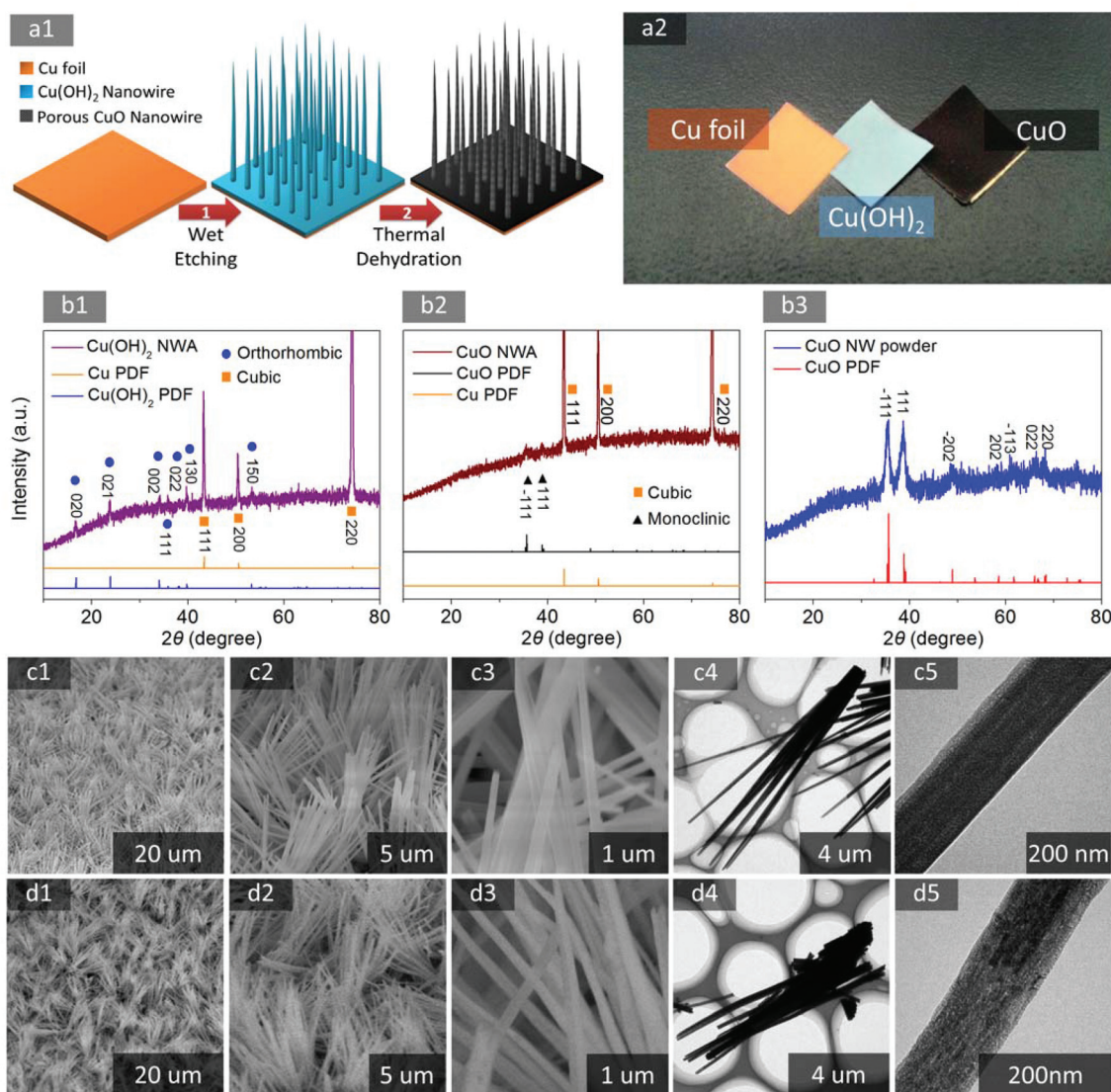
Fig. 1 (a1) Schematic illustration of synthesis of porous CuO NWA on copper foils; (a2) digital photograph of a primitive Cu foil and the foils covered with \text{Cu}(\text{OH})_2 and CuO NWA; XRD patterns of \text{Cu}(\text{OH})_2 NWA (b1), CuO NWA (b2) and CuO NW powders (b3); SEM images of \text{Cu}(\text{OH})_2 NWA (c1 to c3) and CuO NWA (d1 to d3); TEM images of \text{Cu}(\text{OH})_2 NW (c4 to c5) and CuO (d4 to d5) NWs.
