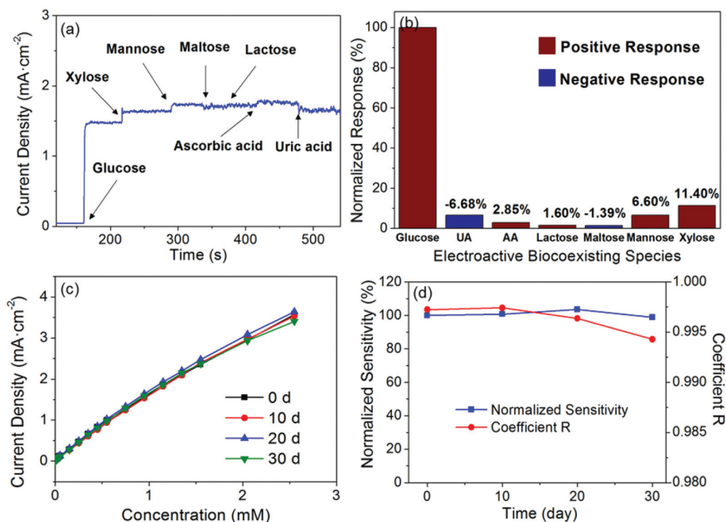
Fig. 6 (a) Amperometric test for selectivity and anti- \text{Cl}^- -poisoning of the NWA sensor and (b) percentage of interfering signals to the target analyte. (c) Calibration plots within the linear range and (d) normalized sensitivity and the corresponding Pearson coefficients of the CuO NWA sensor after different days.
