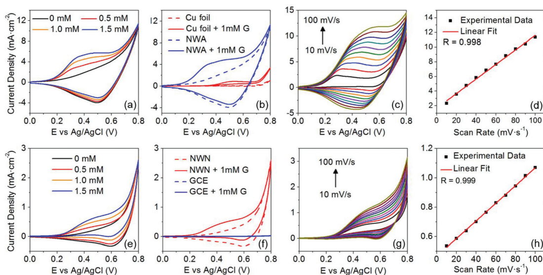
Fig. 2 CV profiles with different concentrations of glucose of (a) CuO NWA and (e) CuO NWP; CV with glucose in absence and presence of (b) CuO NWA compared with planar Cu electrode and (f) CuO NWP compared with GCE; CV at scan rates from 10 to 100 \text{mV s}^{-1} for (c) CuO NWA and (g) CuO NWP in 2.5 mM glucose. (d) The calibration plot of (c). (h) The calibration plot of (g).
