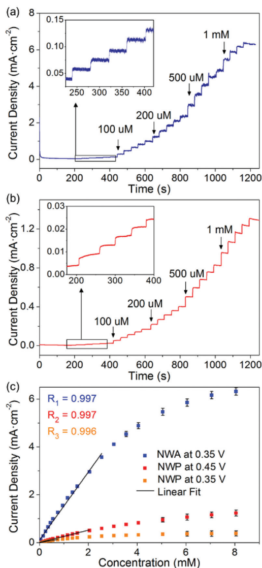
Fig. 4 Amperometric i - t test with successive addition of glucose for the NWA under +0.35 V (a) and the NWP under +0.45 V (b). (c) Calibration plots of (a) and (b). The insets show respective i - t curves at low concentration levels, with stepwise addition of 10 \mu M glucose.
