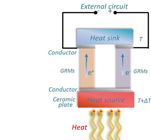
Fig. 105 Schematic illustration of power generation in a TE device based on \text{Bi}_2\text{Te}_3 LMs or GNRs. A T gradient, \Delta T , causes charge carriers in the material to diffuse, resulting in current flow through the external circuit. Adapted from ref. 1841.
