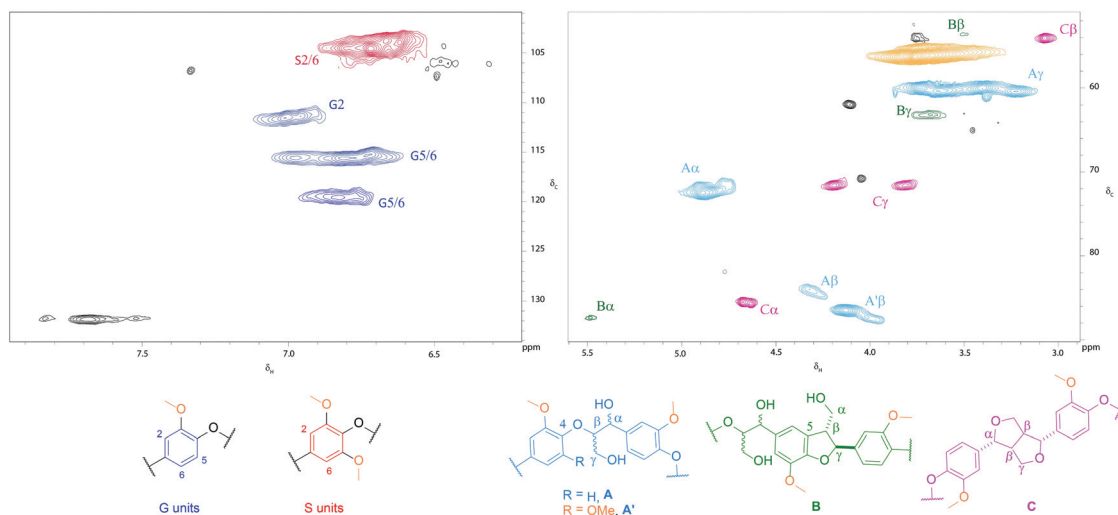
Fig. 1 HSQC NMR spectrum of Poplar ammonia lignin. Contours are colour coded according to the linkage they are assigned to. Black cross peaks correspond to currently unassigned signals. NMR spectra were recorded on a 500 MHz spectrometer at a concentration of 100 mg of the substrate in 0.6 ml of DMSO- d_6 .
