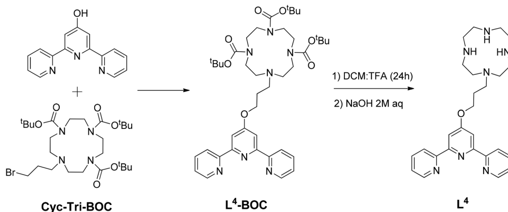
Scheme 1 Reaction scheme for the syntheses of ligand \mathbf{L}^4 .
