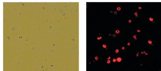
Fig. 95 Top: structure of RHQ probe and related probes 90 and 91 . Bottom: (left) bright field image of PBMCs (40x), (right) fluorescence image of PBMCs (40x) treated with RHQ . Image reproduced with permission. 320
