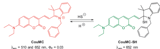
Fig. 53 Structure and reaction of 59 with HS^- .
