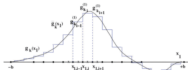
Fig. 8 Approximation of the Gaussian-type basis function by a piecewise constant function.
