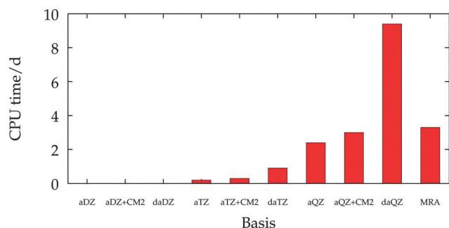
Fig. 5 Total CPU times in days for the calculation of the 10 lowest CIS singlet excitation energies of toluene (50 electrons) in C_1 symmetry with basis sets aug-cc-pVXZ (abbreviated as aXZ) and d-aug-cc-pVXZ (abbreviated as daXZ), as well as MRA.
