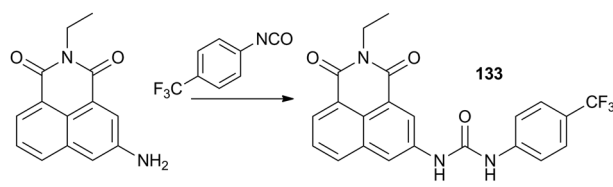
Scheme 15 Synthesis of anion sensor 133 .
