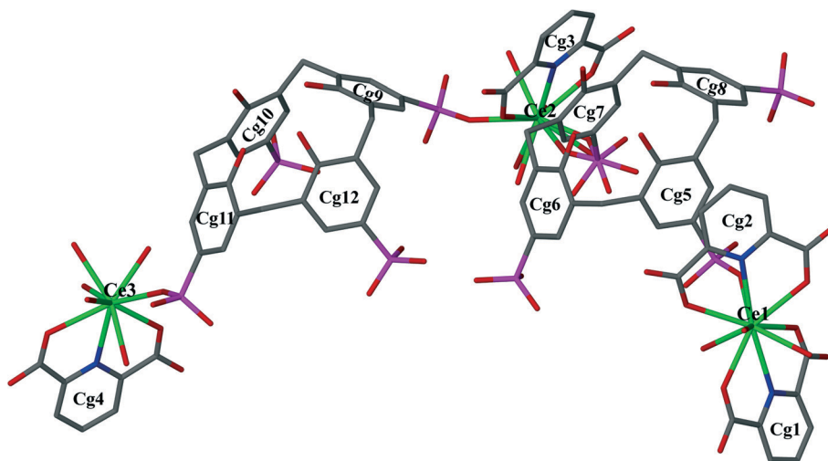
Fig. 1 The asymmetric unit displaying C-shaped supermolecule 1 . Water molecules, nitrate anion and H-atoms have been omitted for clarity. Aromatic rings have been numbered to show centre of gravity. Disorder of the sulfonate group on Cq7 is shown.
