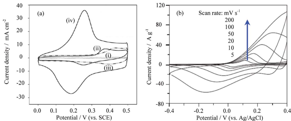
Fig. 14 (a) CV curves of various electrodes at 50 mV s -1 in 1 mol l -1 KOH solution: (i) CNTs; (ii), nickel oxide/CNTs; (iii) cobalt oxide/CNTs; (iv), nickel-cobalt oxides/CNTs (Ni/Co molar ratio = 1 : 1), and (b) CV curves of \alpha -Co(OH) 2 composite electrode recorded in 1 mol l -1 KOH aqueous solution at different scan rates (modified from ref. 84a and 85c).
