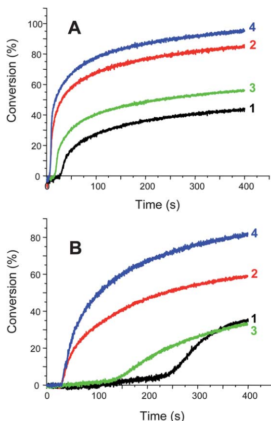
Fig. 6 Photopolymerization profiles of EPOX. (A) upon Xenon lamp irradiation ( \lambda > 390 nm) in the presence of (1) Ru(bpy) 3 2+ /Ph 2 I + (0.2%/2% w/w); (2) Ru(bpy) 3 2+ /TTMSS/Ph 2 I + (0.2%/3%/2% w/w); (3) Ru(phen) 3 2+ /Ph 2 I + (0.2%/2% w/w); (4) Ru(phen) 3 2+ /TTMSS/Ph 2 I + (0.2%/3%/2% w/w). (B) upon a diode laser irradiation (532 nm) in the presence of (1) Ru(bpy) 3 2+ /Ph 2 I + (0.2%/2% w/w); (2) Ru(bpy) 3 2+ /TTMSS/Ph 2 I + (0.2%/3%/2% w/w); (3) Ru(phen) 3 2+ /Ph 2 I + (0.2%/2% w/w); (4) Ru(phen) 3 2+ /TTMSS/Ph 2 I + (0.2%/3%/2% w/w).
