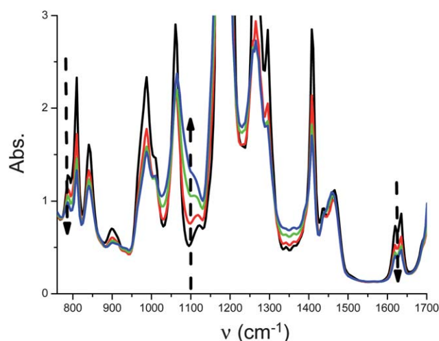
Fig. 7 IR spectra recorded during the photopolymerization of (3,4-epoxycyclohexane)methyl 3,4-epoxycyclohexylcarboxylate/TMPTA (50%/50% w/w) under air in the presence of Ru(phen) 3 2+ /TTMSS/Ph 2 I + (0.1%/3%/2% w/w); fluorescence bulb irradiation at different times ( t = 0 s; 10 s; 40 s and 3 min 30 s). The evolution of the acrylate double bond, epoxide function and polyether group are observed at about 1630\text{ cm}^{-1} , 790 and 1080\text{ cm}^{-1} , respectively.
