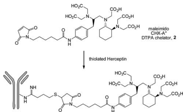
Scheme 31 Conjugation of a maleimide-functional chelator to the monoclonal antibody Herceptin as a facile route to bioconjugates for radioimmunoimaging applications.
