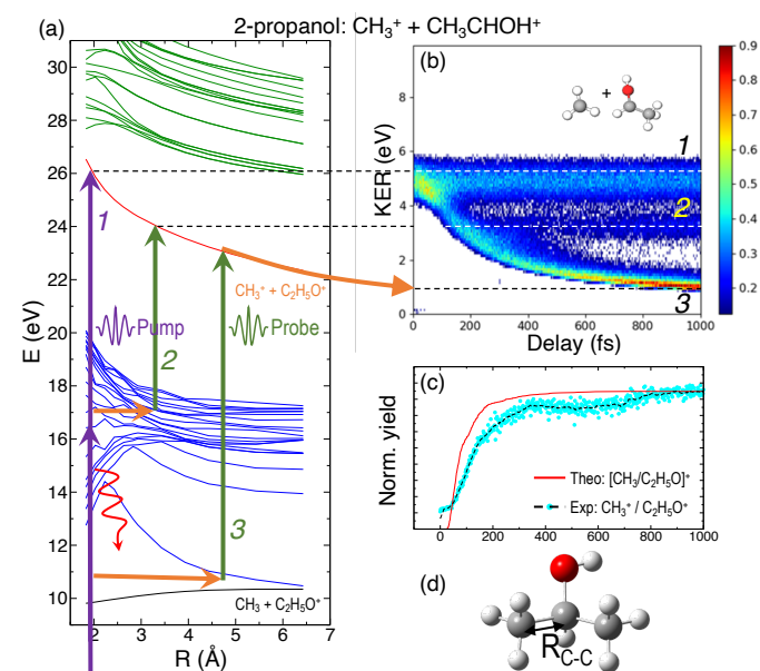
Fig. 2 (a) Potential energy curves of the ground and excited cationic and dicationic states of 2-propanol along the C–C bond shown in the (d). Purple arrows, representing multiphoton absorption induced by the pump pulse, indicate population of electronically excited states. Red curly arrows indicate relaxation to the ground state of the cation, with energy transfer to vibrational modes. (b) Delay-dependent KER for the fragmentation channel \text{CH}_3^+ + \text{CHOHCH}_3^+ . (c) Comparison between the projection of experimentally obtained dynamic KER signal intensity and theoretical yield using E_{\text{exc}} = 10 eV for the fragmentation channel.
