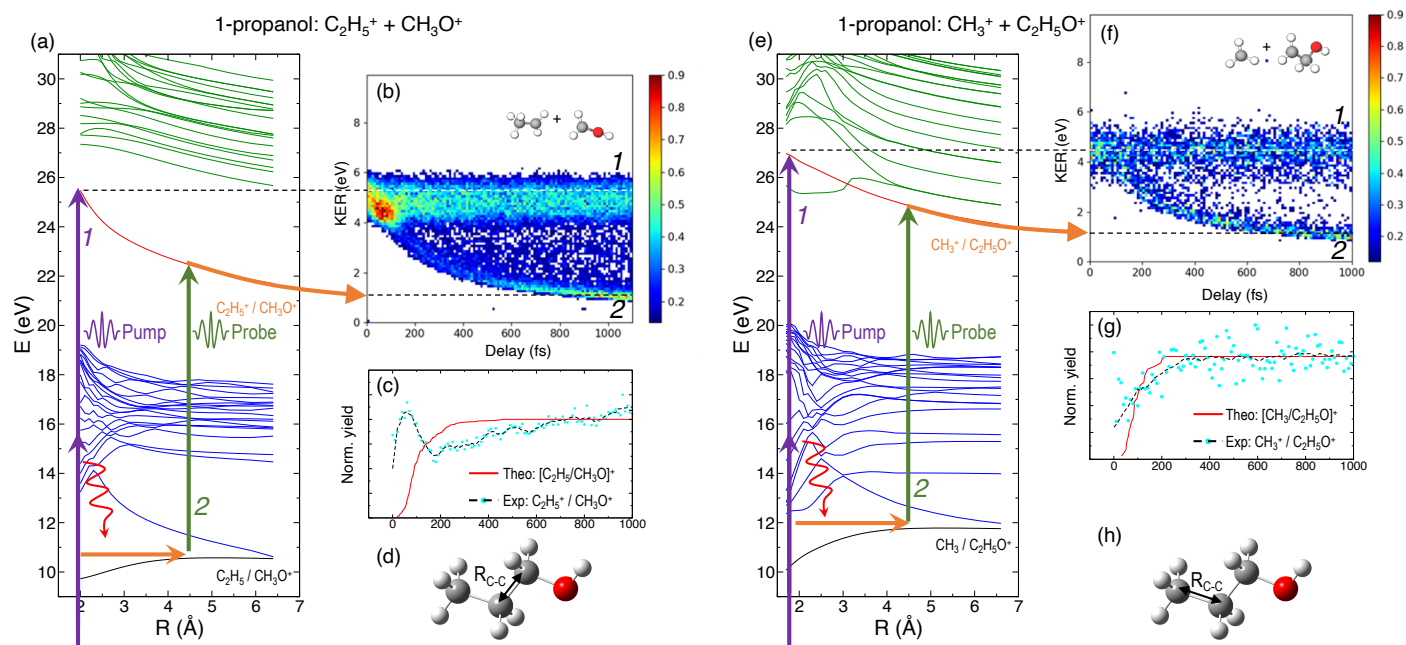
Fig. 1 (a), (e) Potential energy curves showing the ground and excited cationic and dicationic states of 1-propanol along the C–C bonds indicated in the ball-and-stick models shown in (d) and (h), respectively. Purple arrows, representing multiphoton absorption induced by the pump pulse, indicate population of electronically excited states. Red curly arrows indicate relaxation to the ground state of the cation, with energy transfer to vibrational modes. Kinetic energy release as a function of the time delay between the pump and probe pulses for the double coincidence fragmentation channels (b) \text{C}_2\text{H}_5^+ + \text{CH}_2\text{OH}^+ and (f) \text{CH}_3^+ + \text{C}_2\text{H}_4\text{OH}^+ of 1-propanol. (c), (g) Comparison between the projection of experimentally obtained dynamic KER signal intensities and theoretical yields using E_{\text{exc}} = 10 eV for the corresponding channels.
