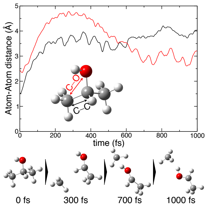
Fig. 7 A typical trajectory of the molecular dynamics simulations showing methyl roaming. The upper plot shows C–O and C–C bond distances as a function of the time. The lower part shows snapshots of methyl roaming at different propagation time.
