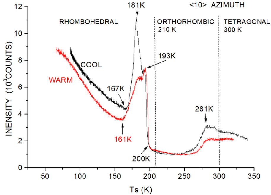
Surface temperature scan of the 52% Nb KTN target in the \langle 10 \rangle azimuth. The specular He scattering intensity yielded the upper curve as the target was cooled from \sim 350 K to \sim 80 K and the lower curve as it was warmed from \sim 60 K to \sim 325 K. The He atom wave vector k_i = 7.88 \text{ \AA}^{-1} . The dotted vertical lines indicate the bulk phase transitions.
