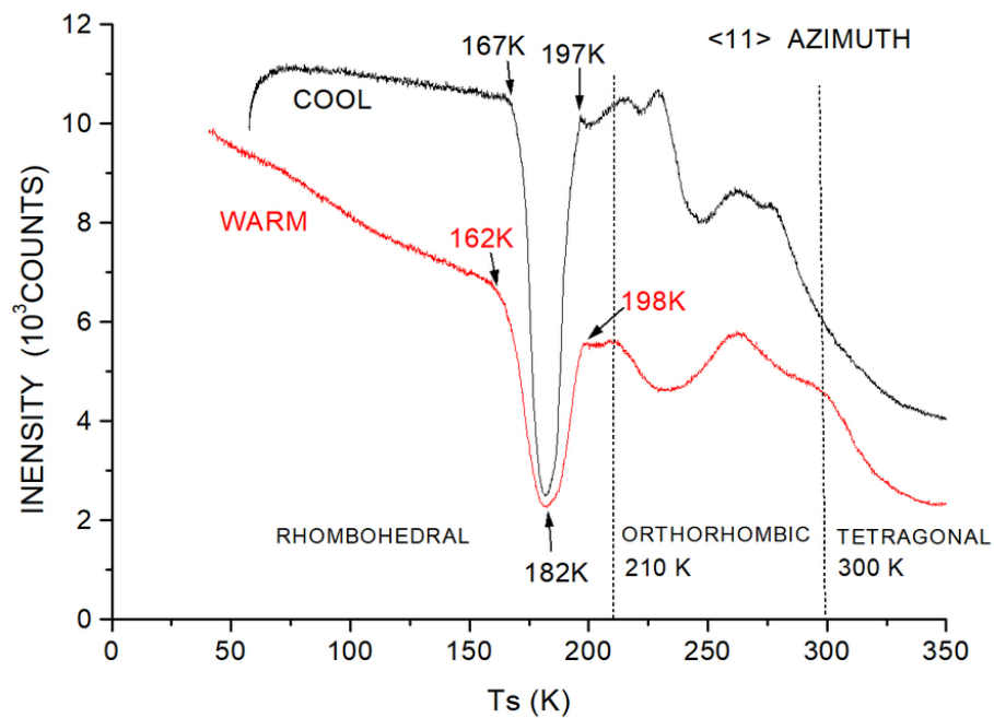
Surface temperature scan of the 52% Nb KTN target in the <11> azimuth. The scans were carried out as in Figure 4 with upper cooling curve from \sim 350\text{K} to \sim 60\text{K} and lower warming curve from \sim 50\text{K} to \sim 350\text{K} . The initial He atom wave vector k_i = 7.48\text{\AA}^{-1} . The dotted vertical lines indicate the bulk phase transitions.
