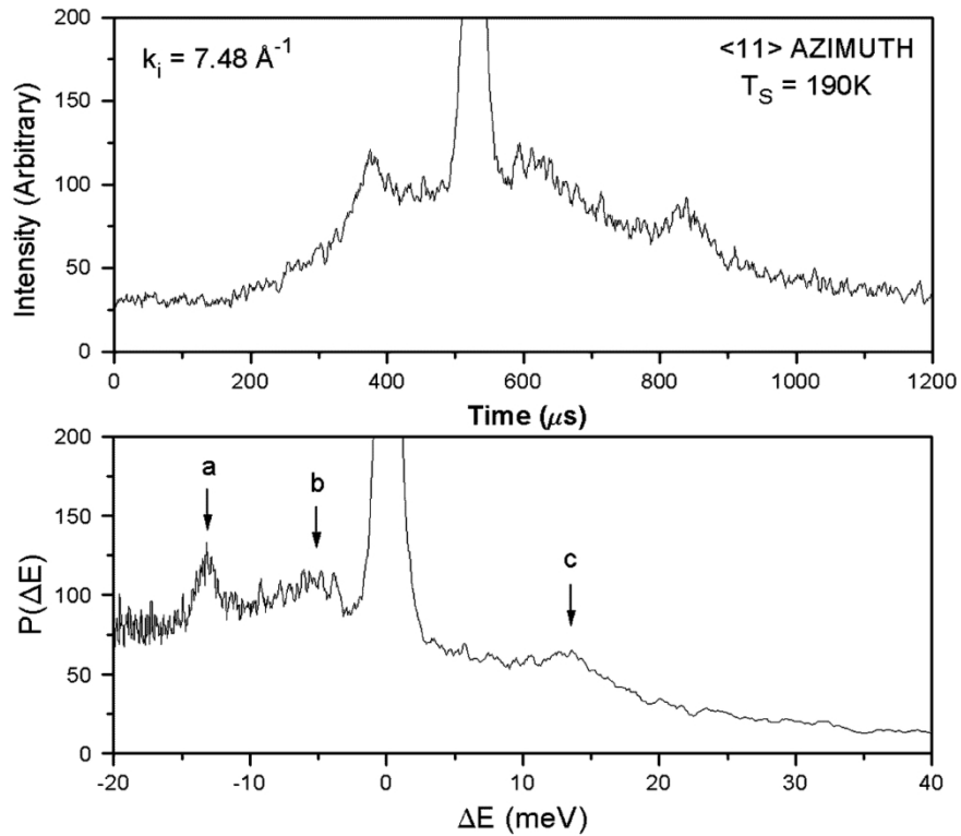
Time of flight spectrum of the 52% Nb KTN target at a surface temperature of 190K in the \langle 11 \rangle azimuth taken at an incident angle of 42^\circ . The upper panel shows the arrival time spectrum. The lower panel shows the transform of the upper panel into an energy transfer spectrum. The peaks a, b, and c are at energies -13.5, -5.0, 14.0 meV respectively.
