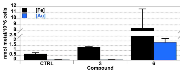
Figure 4. ICP-MS detection of intracellular Fe and Au levels from A549 cells treated with compounds 3 and 6 . Error bars represent one standard deviation. Although a biological trend is evident, statistical analysis (i.e., one-way ANOVA) resulted in a P value of 0.09. This result may be explained by our small sample size (N=2).
