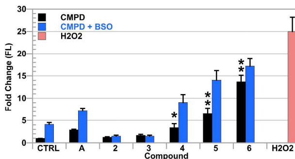
Figure 5. Reactive oxygen species detected by fluorescent signal increases of DCF via flow cytometric analysis in live A549 cells treated with various complexes. H 2 O 2 was used as a positive control. Error bars represent one standard deviation. A one-way ANOVA with Dunnet's post-hoc test was used to compare each compound with the vehicle control (* P<0.05; ** P<0.01).
