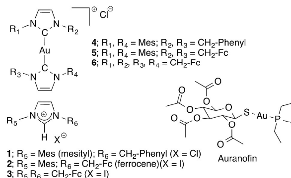
Figure 1. Ferrocene containing imidazolium salts ( 1–3 , previous work), their corresponding [Au(NHC) 2 ] + gold(I) complexes ( 4–6 , this work), and control complex auranofin studied for their abilities to disrupt antioxidant pathways, generate ROS, and inhibit cell proliferation.
