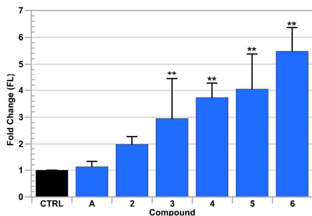
Figure 7. Detection of intracellular zinc fluctuations by fluorescent signal increases of FluoZin-3 via flow cytometric analysis in live A549 cells treated with various complexes. Error bars represent one standard deviation. A one-way ANOVA with Dunnet's post-hoc test was used to compare each compound with the vehicle control (** P < 0.01 ).
