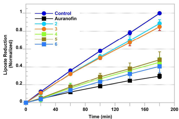
Figure 6. Time-dependent inhibition of thioredoxin reductase (TrxR) via the reduction of lipoate. Error bars represent standard deviation. For clarity, statistical symbols were not included in this figure. A one-way ANOVA with Dunnet's post-hoc test was used to compare TrxR activity at the 180-minute time point. At this time point, all compounds were statistically different from the control (P<0.05: 2 and 3 ; P<0.001: Auranofin, 4 , 5 , and 6 ) and Auranofin (P<0.05: 5 and 6 ; P<0.001: 2 , 3 , and 4 ) in their ability to inhibit TrxR.
