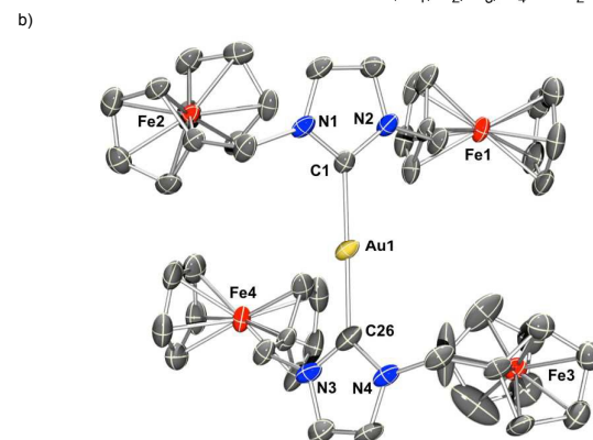
Figure 2. a) Synthesis of ferrocene containing Au(I) carbene complexes. b) ORTEP diagram of 6 rendered using POV-Ray. Thermal ellipsoid plots are drawn at the 50% probability level. Hydrogen atoms and counter anion are omitted for clarity. Selected bond lengths ( \text{\AA} ) and angles (deg): C1–N1, 1.37(1); C1–N2, 1.35(2); C1–Au1, 2.021(9); C26–Au1, 2.028(8); C26–N3, 1.33(1); C26–N4, 1.35(1); N1–C1–N2, 105.2(8); N3–C26–N4, 105.1(7); C1–Au1–C26, 176.5(3).
