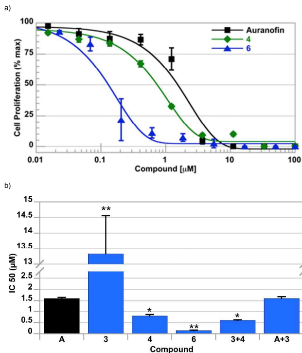
Figure 3. a) Cell proliferation profiles and b) Bar graph plot summarizes the potency of all the compounds explored. Note that the potency of 6 is greater than the 2:1 mixture of compounds 3 and 4 . Error bars represent one standard deviation. A one-way ANOVA with Dunnet's post-hoc test was used to compare each compound with Auranofin (* P < 0.05 ; ** P < 0.01 ).
