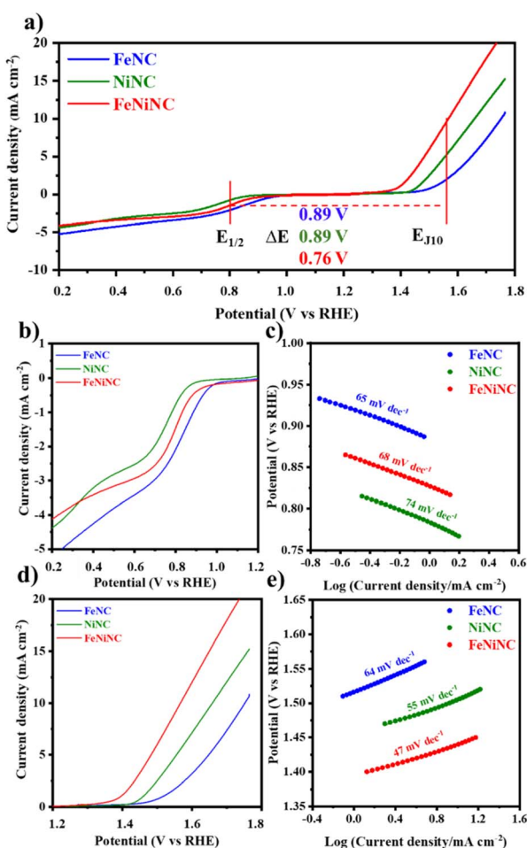
Fig. 4 LSV with an RDE at a scan rate of 10 \text{ mV s}^{-1} and rotation speed of 1600 rpm in \text{O}_2 -saturated ( 0.1 \text{ M} ) KOH electrolyte: (a) overall LSV polarization curve, (b) LSV curve for the ORR and (c) corresponding Tafel plots, (d) LSV curves for the OER and (e) corresponding Tafel plot of FeNC (blue), NiNC (green) and FeNiNC catalysts (red).
