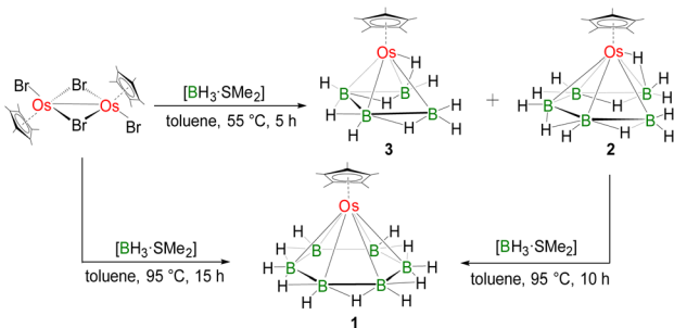
Scheme 1 Synthesis of 1 [Cp*Os(η 6 -B 6 H 11 )], 2 [Cp*Os(η 5 -B 5 H 12 )], and 3 [Cp*Os(η 4 -B 4 H 9 )].
