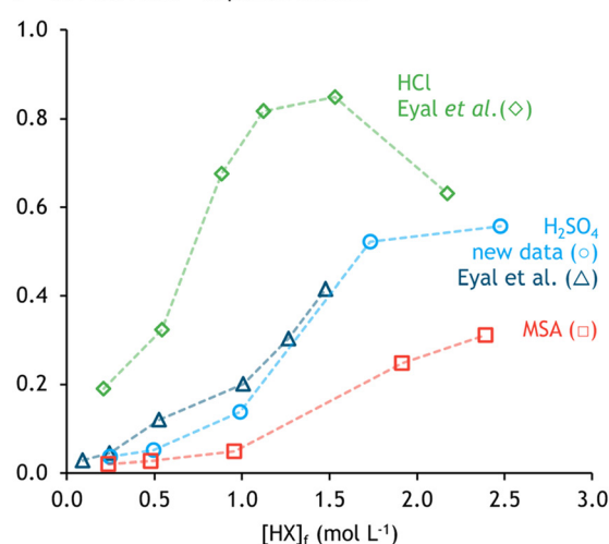
Fig. 3 Solvent extraction data of H 2 SO 4 , HCl, and MSA – TEHA + dodecane systems at 25 °C. Graph c compares this to literature data from Eyal et al. 46 Distribution ratios are shown for three TEHA concentrations with varying H 2 SO 4 concentrations in the feed (a), and with varying initial TEHA concentrations in the solvent (b). (c) Compares the extraction of HCl, H 2 SO 4 , MSA by 43 vol% TEHA.
