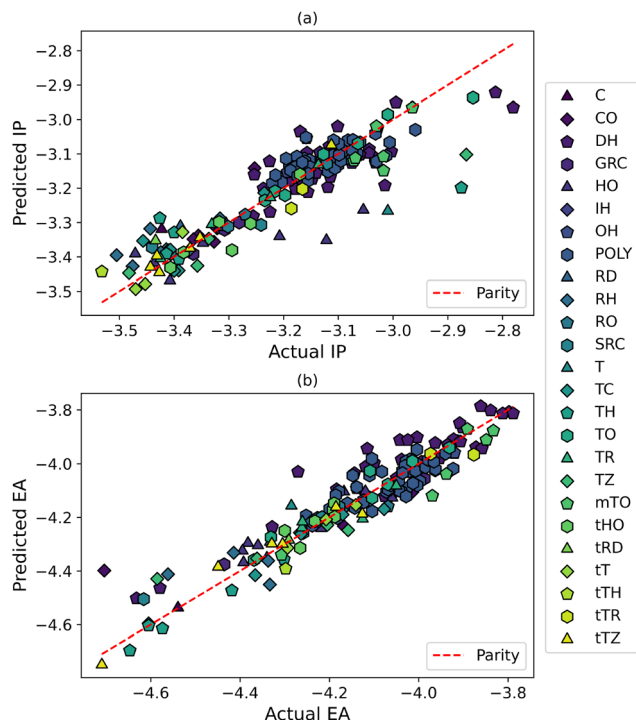
Fig. 3 Model testing results predicting (a) the ionisation potential (IP) and (b) the electron affinity (EA) for Au nanoparticle morphologies listed in Table 1, using the S descriptor describing the structure of the surfaces of the nanoparticles.
