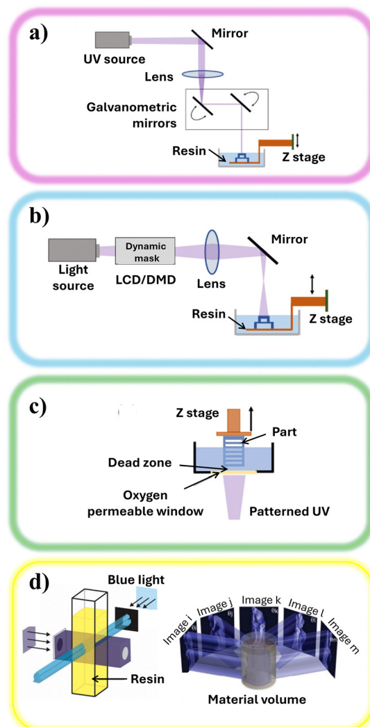
Fig. 15 Scheme of: (a) scanning laser beam; (b) projection stereolithography; (c) liquid interface production; (d) volumetric stereolithography. Reproduced with permission from ref. 374. Copyright 2020 MDPI.
