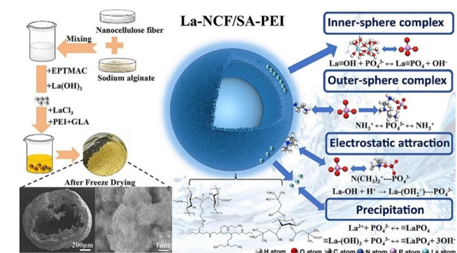
Fig. 2 Schematic representation of the synthesis process of the La-NCF/SA-PEI hydrogel and its morphology and P removal and recovery via inner-sphere complex, outer-sphere complex, electrostatic and precipitation mechanisms (reprinted with permission from Zhang et al. ). 58
