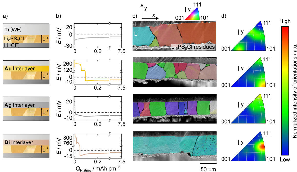
Fig. 1 Electrodeposition of lithium using (a) different interlayer materials. (b) Voltage profiles of the respective cell systems ( T = 25\ ^\circ\text{C} , j = 150\ \mu\text{A cm}^{-2} ). As schematically depicted, titanium was used as reference (top row) and gold (2nd row), silver (3rd row) and bismuth (4th row) were used as interlayer materials. (c) Microstructure of the electrodeposited lithium layers using the different interlayer materials. The IPF maps are given parallel to the y -direction as indicated above. The shown scalebar represents 50\ \mu\text{m} in all cases. (d) IPFs of the analyzed cross-sections showing the distribution of the orientation of all analyzed grains. The IPFs are given parallel to the y -direction. Please note that the IPFs were created based on the entire analyzed cross-section, which is shown in the SI.
