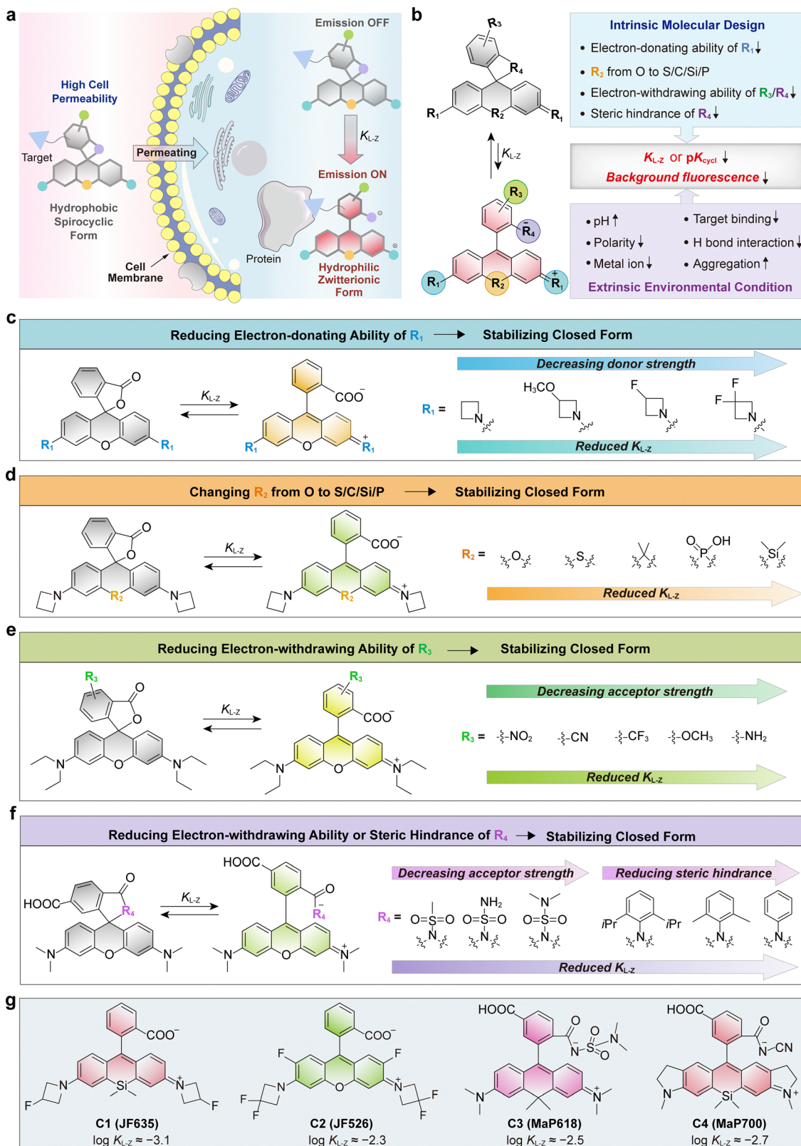
Fig. 18 (a) Schematic illustration of protein labeling-induced ring opening of rhodamines, converting the closed, non-emissive spiroactone (or spiroactam) form into the open, zwitterionic or cationic emissive form. (b) Intrinsic molecular design strategies and extrinsic factors that favor the spirocyclization equilibrium toward the closed form of rhodamines. (c)–(f) Various molecular design strategies to stabilize the closed form of rhodamines. (g) Chemical structures of representative rhodamines and their \log K_{L-Z} values.
