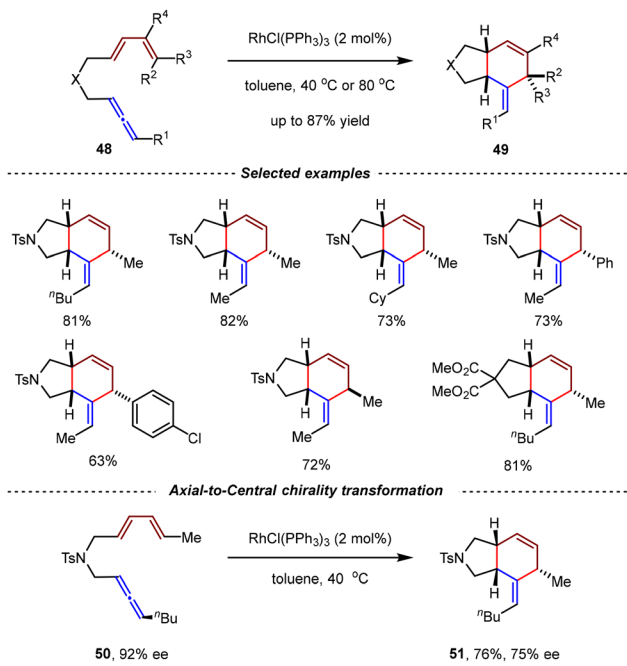
Scheme 15 RhCl(PPh 3 ) 3 -catalyzed intramolecular [4+2] cycloadditions of 1,3-disubstituted allene-1,3-dienes.
