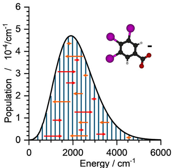
Fig. 7 Single well without dissociation: population for \text{C}_6\text{H}_2\text{I}_3\text{COO}^- at 300 K in stationary state. Red arrows indicate photon absorption, orange arrows photon emission. Both processes shift population from one energy bin to another. In the stationary state, these shifts exactly cancel out.
