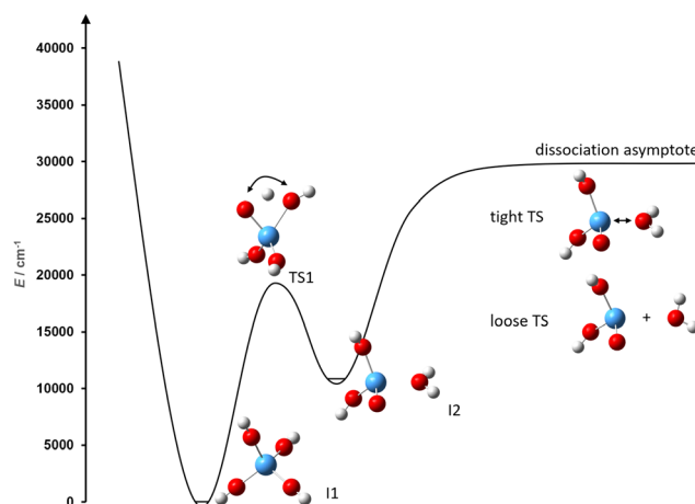
Fig. 1 Isomerization of \text{Ta}(\text{OH})_4^+ via TS1 to \text{TaO}(\text{OH})_2(\text{H}_2\text{O})^+ , followed by loss of \text{H}_2\text{O} , which may be represented by a tight or loose TS, calculated at the B3LYP/def2-TZVPP level of theory. See animated GIFs of TS1 and tight TS available as SI.
