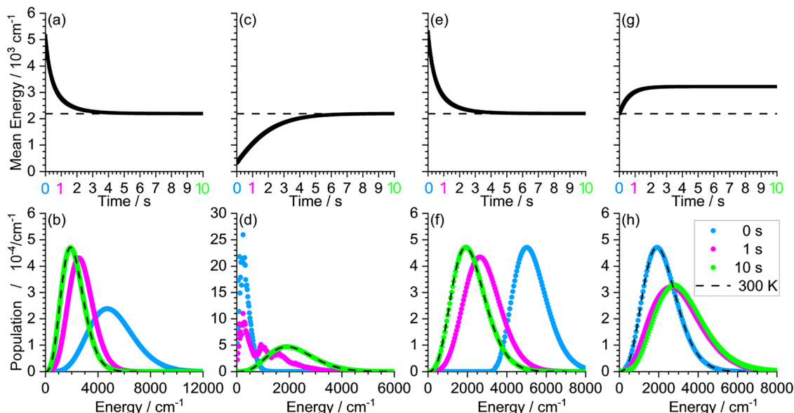
Fig. 8 MEM of \text{C}_6\text{H}_2\text{I}_3\text{COO}^- simulating changes in internal energy in a 300 K environment: (a) and (b) cooling of an initial 500 K population; (c) and (d) heating of an initial 100 K population; (e) and (f) equilibration of a 300 K population after absorption of a 3091.43\text{ cm}^{-1} photon; (g) and (h) IRMPD experiment with absorption of 1694.44\text{ cm}^{-1} photons at a rate of 1 photon per second.
