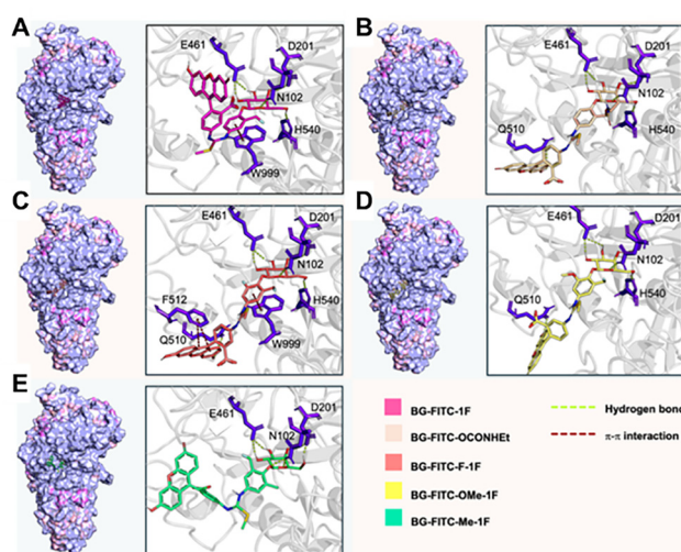
Fig. 3 The interaction map of the complex of Escherichia coli \beta -Gal (PDB: 1JYX) with (A) BG-FITC-1F , (B) BG-FITC-OCONHt , (C) BG-FITC-F-1F , (D) BG-FITC-OMe-1F , or (E) BG-FITC-Me-1F . The amino acids shown have interactions with the probe molecule.
