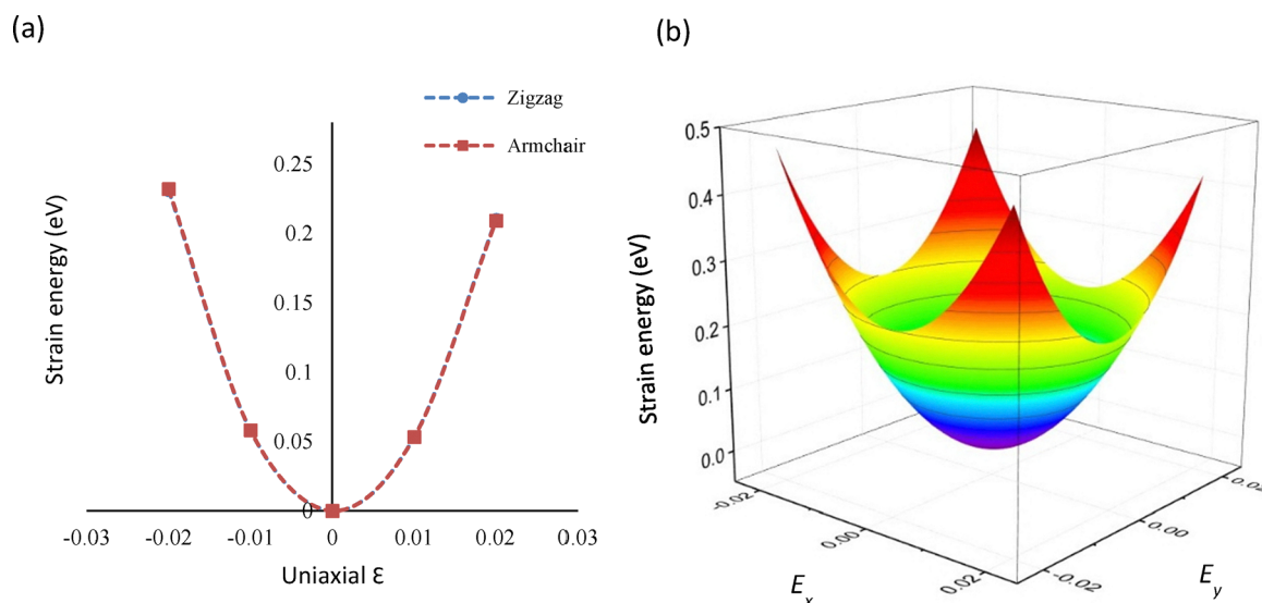
Fig. 4 Structural and mechanical response of the 2D VS 2 /Gr composite under uniform expansion: (a) uniaxial strain energy-strain curves along the armchair and zigzag directions and (b) 3D fitted surface plot of total energy as a function of elastic strain.
