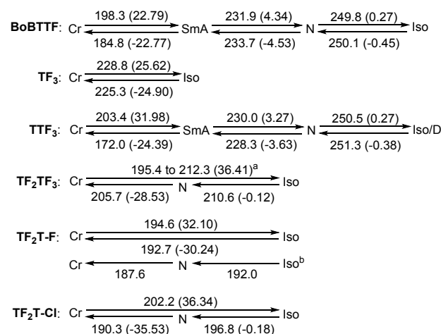
Figure 5. Phase transition temperatures (°C) and enthalpies (kJ mol -1 ) of derivatives with the bithiophene moiety ( TT ) partially or fully fluorinated. Values are determined by DSC at 5 °C/min under N 2 for 2 nd -heating and 1 st -cooling runs). Cr = crystalline phase; SmA = smectic A; N = nematic; Iso = isotropic liquid; D = decomposition. a Broad melting transition with several overlapping peaks; Values given are the onsets of the transitions for the first and last thermal event. b Observed only by POM at high cooling rates >20 °C/min.
