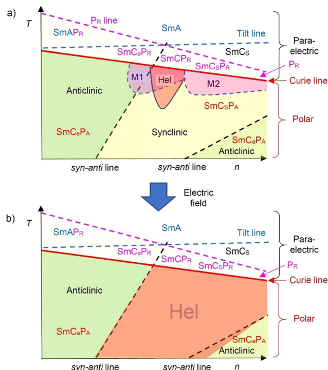
Fig. 18 Sketch of the development of tilt, polar order and helicity in the smectic LC phases of the bent-core molecules 1/On depending on temperature and alkyl chain length ( n = 8-20 ): (a) in the pristine material and (b) after applying a short AC sequence; Hel = heliconical \text{Sm}(\text{CP})^{\text{hel}} phase, for other abbreviations, see Table 2.
