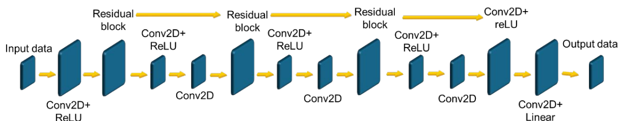
Figure 2. Architecture of the SRCNN model utilized in this study, illustrating the convolutional and residual layers.
