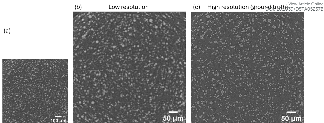
Figure 1. (a) Example of experimental low-resolution image of NMC811 cathode acquired at 2.3 μm per pixel, (b) corresponding scaled-up version of the low-resolution image, and (c) experimental high-resolution image obtained at 0.74 μm per pixel.
