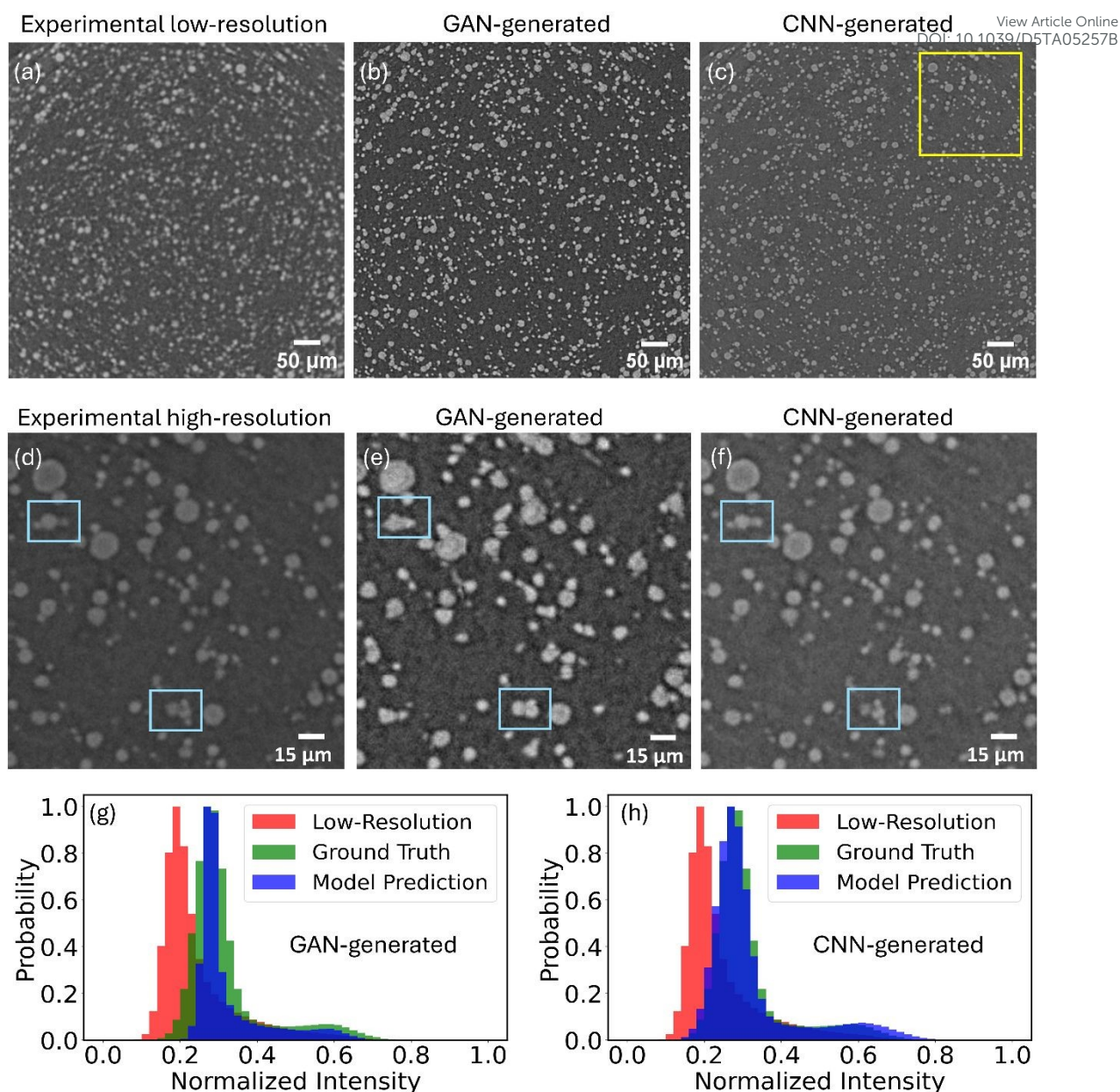
Figure 5. (a) Experimental low-resolution image. (b) GAN model-generated; and (c) CNN model-generated high-resolution images. The yellow square in (c) shows the position of the zoom-in section in (d-f). Cropped section to show the zoomed-in section of (d) experimental high-resolution image (ground truth); (e) GAN model-generated; and (f) CNN model-generated high-resolution images. The term zoomed-in does not indicate optical magnification but rather cropped regions (highlighted by the yellow box in Figure 5c) to allow easier comparison of the fine details in the images. The blue rectangles in (d-f) indicate the same regions for better comparison. Normalized histograms of intensity distributions for experimental low-resolution, experimental high-resolution (ground truth), and predicted images by (g) GAN; and (h) CNN.
