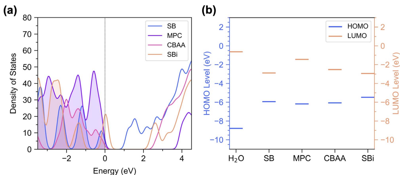
Fig. 2 Electronic properties of zwitterionic polymers: (a) total electronic density of states of the four polymers. (b) Calculated HOMO–LUMO energy levels vs. vacuum.
