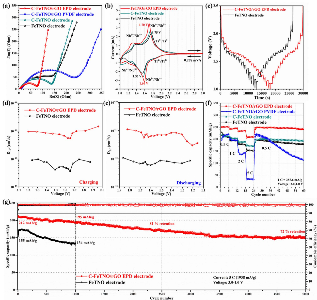
Fig. 5 (a) EIS, (b) CV, (c) GITT and D_{Li^+} of the C-FeTNO/rGO EPD electrode and the FeTNO electrode during (d) charging and (e) discharging. (f) Rate performance of the C-FeTNO/rGO EPD electrode, C-FeTNO/rGO PVDF electrode, C-FeTNO electrode, and FeTNO electrode, (g) long cycling performance of the C-FeTNO/rGO EPD electrode and the FeTNO electrode.
