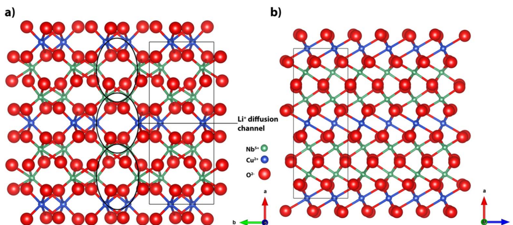
Fig. 1 (a) Front view and (b) side view of the orthorhombic CuNb 2 O 6 columbite crystal structure. Elements are shown with their ionic radii, the Li + -diffusion channels are only open in the \langle 0\ 2\ 1 \rangle vector, and fully closed along the \langle 0\ 0\ 1 \rangle vector.
