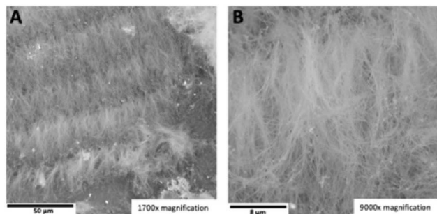
Fig. 4 DAC Genesis CNT products formed at \text{CO}_2 sufficient conditions. 750 ^\circ\text{C} \text{Li}_2\text{CO}_3 electrolyte electrolysis with a brass cathode and a stainless steel anode and case. SEM of the washed products: CNTs (A & B) 1700 \times and 9000 \times magnification.
