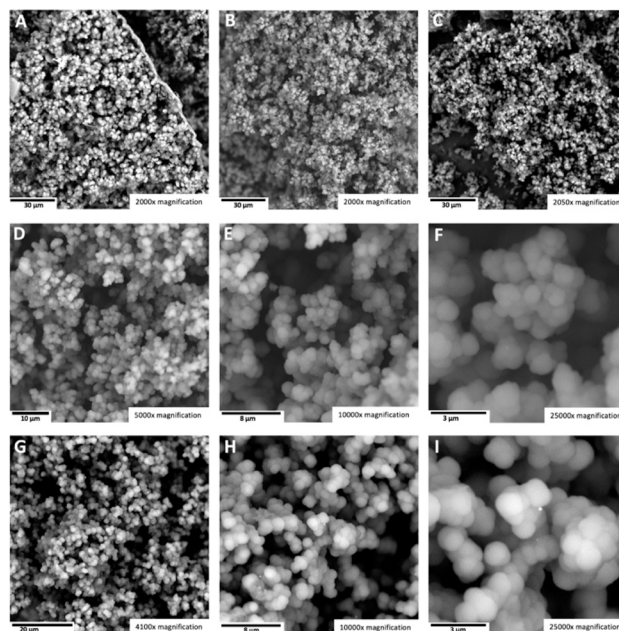
Fig. 5 DAC Genesis CNO products formed at \text{CO}_2 insufficient conditions. 750 ^\circ\text{C} \text{Li}_2\text{CO}_3 electrolyte electrolysis with a brass cathode and a stainless steel anode and case. SEM of the washed products: CNOs sample 1 (A–F) magnification at 2000 \times , 2000 \times , 2050 \times , 5000 \times , 100 00 \times , 250 00 \times . CNOs sample 2 (G–I) 4100 \times , 10 000 \times , and 250 00 \times .
