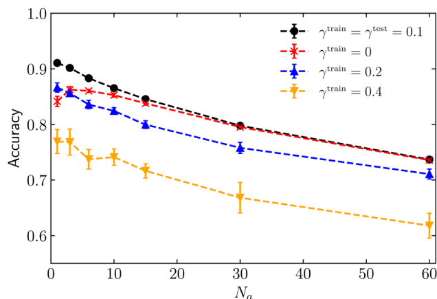
Fig. 6 Accuracy as a function of the number of active cells N_a for neural networks solely trained on local shape features. The black dots represent accuracy obtained from individual models, each trained using \gamma^{\text{train}} = \gamma^{\text{test}} = 0.1 . The red stars, blue triangles, and orange inverted triangles represent accuracy obtained from models trained with data for \gamma = 0 , \gamma = 0.2 or \gamma = 0.4 , respectively. The accuracy for each of these lines corresponds to the neural network tested on \gamma = 0.1 .
