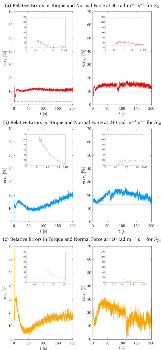
Fig. 8 Relative errors in the torque \text{err}_\tau and force \text{err}_{N_z} for samples (a) S_2 , (b) S_{16} and (c) S_{24} at twist rates of \{40, 240, 400\} \text{ rad m}^{-1} \text{ s}^{-1} . The insets show the ramp phase in more detail. The dashed lines indicate the relative errors at the end of the ramp phase.
