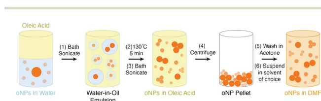
Fig. 1 Schematic of the solvent-transfer process.
