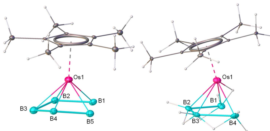
Fig. 3 Molecular structures of ( 2 ) \text{Cp}^*\text{Os}(\eta^5\text{-B}_5\text{H}_{12}) (left) and ( 3 ) (\text{Cp}^*\text{Os})(\eta^4\text{-B}_4\text{H}_9) (right). Hydrogen positions in 2 could not be located crystallographically due to disorder. They were confirmed by different NMR experiments and computational analysis. Selected bond lengths (Å) and angles (deg.) for 2 : Os1–B2 2.02(3), Os1–B3 2.15(3), Os1–B5 2.16(3), Os1–B4 2.23(3), Os1–B1 2.24(3), B1–B2 1.77(4), B3–B4 1.77(4); B2–Os1–B3 57.0(12), B3–Os1–B5 81.9(17), B1–B3 118(3), B4–B2 118(3), B5–B3 107(3). Selected bond lengths (Å) and angles (deg.) for 3 : B1–B2 1.846(11), B2–B3 1.826(12), B3–B4 1.851(13), Os1–B1 2.305(7), Os1–B2 2.146(7), Os1–B3 2.150(7), Os1–B4 2.300(7); B3–B1 111.7(6), B2–B4 112.4(5).
