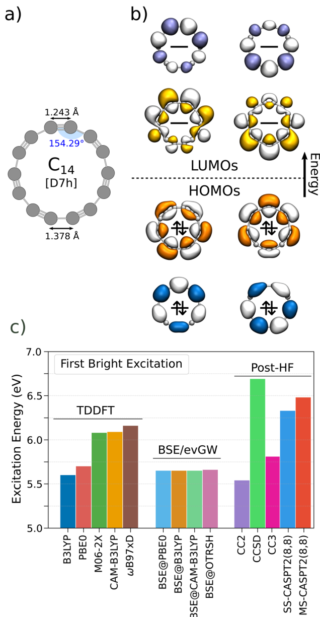
Fig. 1 (a) Molecular structure of C_{14} . Geometric parameters (bonds and angles) at the CCSD/cc-pVDZ level 13 and point group symmetry are highlighted; (b) graphical depiction of the eight valence MOs involved in the first bright transition of C_{14} , calculated at the HF/aug-cc-pVDZ level (dark: occupied MOs, light: virtual MOs). (c) C_{14} excitation energies (eV) of the first bright transition as a function of the level of theory.
