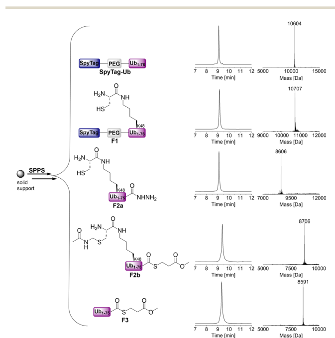
Fig. 3 Synthesis of SpyTag-Ub and the required building blocks for the preparation of the SpyTag-Ub variants using SPPS. Calculated masses: SpyTag-Ub: 10 606 Da, F1 : 10 709 Da, F2a : 8606 Da, F2b : 8706 Da, F3 : 8591 Da.
