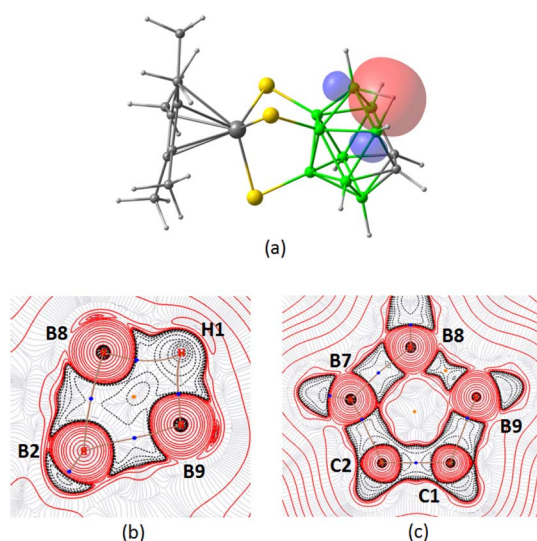
Fig. 8 (a) Selected NBO of 5 showing the 3c–2e interaction of B8–H1–B9 (isocontour values: \pm 0.045\text{ [e bohr}^{-3/2}] ). Contour-line diagram of the Laplacian of the electron density along (b) B8–H1–B9 and (c) B7–B8–B9 planes in 5 .
