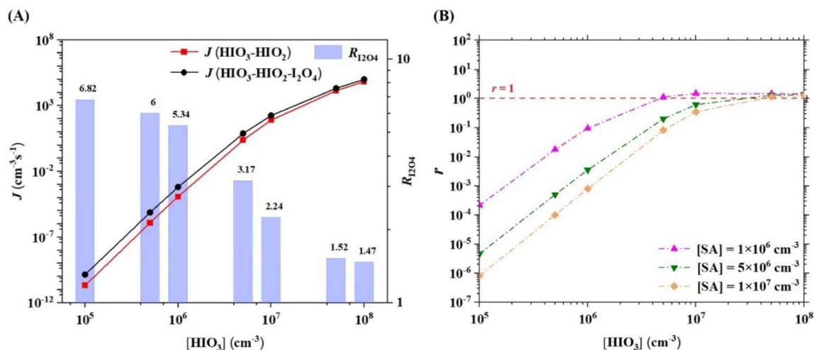
Fig. 4 Cluster formation rates ( J ) (cm -3 s -1 ) of the \text{HIO}_3\text{-HIO}_2 and \text{HIO}_3\text{-HIO}_2\text{-I}_2\text{O}_4 systems and enhancement coefficient ( R_{\text{I}_2\text{O}_4} ) (the ratio of the J value of the \text{HIO}_3\text{-HIO}_2\text{-I}_2\text{O}_4 system relative to that of the \text{HIO}_3\text{-HIO}_2 system) (A) and comparison coefficient ( r ) (the ratio of the J value of the \text{HIO}_3\text{-HIO}_2\text{-I}_2\text{O}_4 system relative to that of the \text{SA-HIO}_3\text{-HIO}_2 system) (B) as a function of precursor concentration at 278.15 K, 1 atm and k_{\text{coag}} = 0.002 \text{ s}^{-1} .
