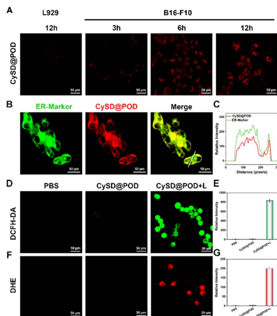
Fig. 4 (A) Confocal fluorescence images of CySD@POD incubation in L929 and B16-F10 cells at different time points. (B) Confocal fluorescence images of B16-F10 cells co-stained with CySD@POD (5 \mu\text{M} , \lambda_{\text{ex}} = 561 nm and \lambda_{\text{em}} = 600 \pm 26 nm) and commercial dyes ER Tracker Green (0.5 \mu\text{M} , \lambda_{\text{ex}} = 488 nm and \lambda_{\text{em}} = 525 \pm 25 nm). (C) Linear analysis of selected regions in confocal fluorescence images. (D) Detection of intracellular ROS in B16-F10 cells using DCFH-DA ( \lambda_{\text{ex}} = 488 nm and \lambda_{\text{em}} = 525 \pm 25 nm). (E) Quantification of green fluorescence intensity from DCFH-DA stained fluorescence images. (F) Detection of intracellular \text{O}_2^{\cdot-} in B16-F10 cells using DHE ( \lambda_{\text{ex}} = 561 nm and \lambda_{\text{em}} = 750 \pm 50 nm). (G) Quantification of red fluorescence intensity from DHE stained fluorescence images. Scale bar: 50 \mu\text{m} . Laser: 750 nm, 0.1 W \text{cm}^{-2} , 5 min.
