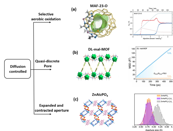
Fig. 6 (a) Crystal and pore structures of MAF-23-O, and breakthrough curves and adsorption kinetic curves using an equimolar C 3 H 6 /C 3 H 8 mixture at 298 K and 1 atm. (b) Structure of DL -mal-MOF and MD-derived self-diffusion rates of C 3 H 6 and C 3 H 8 . (c) Three-dimensional structure of ZnAtzPO 4 and distribution of the aperture size of the bottleneck. Reprinted with permission from ref. 88. Copyright 2019 John Wiley & Sons, ref. 27. Copyright 2023 The American Chemical Society, ref. 35. Copyright 2020 Science, respectively.
