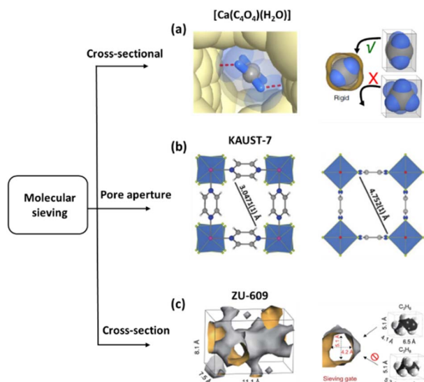
Fig. 5 (a) Preferential binding site for C 2 H 4 molecules, and size/shape sieving based on the minimum cross-sectional areas of C 2 H 4 and C 2 H 6 molecules. (b) Crystal structure of NbOFFIVE-1-Ni, and simulation of the maximum open structure of NbOFFIVE-1-Ni. (c) Sieving gate of ZU-609 and the molecular sizes of propylene and propane. Reprinted with permission from ref. 70. Copyright 2018 Springer Nature Limited, ref. 32. Copyright 2016 The American Association for the Advancement of Science, ref. 33. Copyright 2023 The American Association for the Advancement of Science, respectively.
