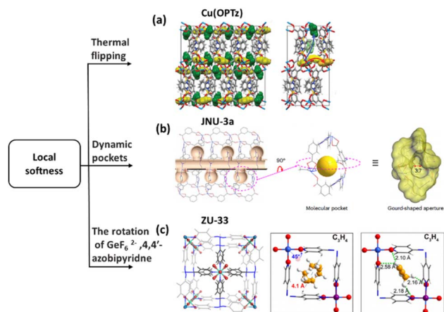
Fig. 10 (a) Simulation of the structure of activated Cu(OPTz)-loaded C_2H_4 and the diffusion structure between the interlayer and intralayer. (b) Crystal structure of JNU-3a with molecular pockets and schematic diagram of molecular pockets. (c) The structure of ZU-33 and bonding sites for loaded C_3H_4 and C_3H_4(PD) . Reprinted with permission from ref. 72. Copyright 2019 American Association for the Advancement of Science, ref. 106. Copyright 2024 Springer Nature Limited, ref. 107. Copyright 2022 Springer Nature Limited, respectively.
