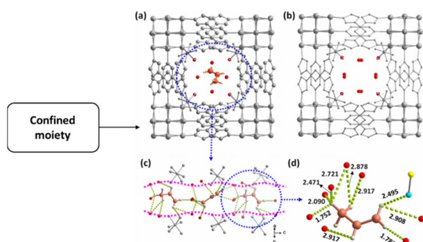
Fig. 11 Crystal structure of loaded C_3H_6 and C_3H_8 samples: (a) NTU-85-WNT \supset C_3H_6 and (b) NTU-85-WNT \supset C_3H_8 and (c, d) detailed H-bonding interactions of C_3H_6 in one-dimensional nanochannels. Reprinted with permission from ref. 37. Copyright 2023 American Chemical Society.
