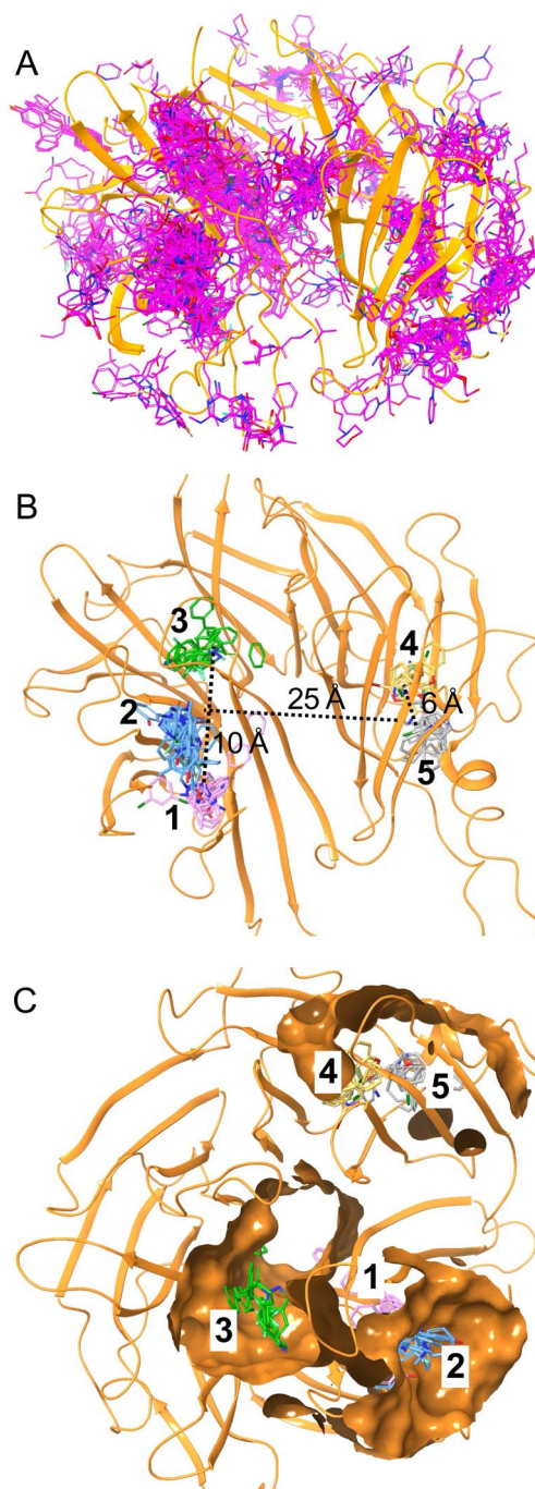
Fig. 1 FRASE database screening. (A) 2544 ligand fragments (magenta sticks) seeded in the LRRK2 WDR structure (orange ribbons); (B) 85 ligand fragments with scores >0.4 are grouped into five distinct clusters (1–5); (C) potential ligand-binding pockets corresponding to clusters 1–5.
