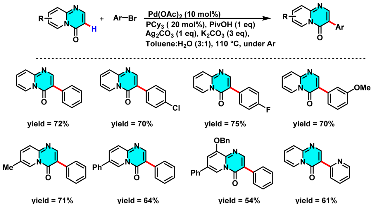
Scheme 7 \text{Pd}(\text{II}) -catalyzed synthesis of 3-aryl-pyrido[1,2- a ]pyrimidin-4-ones in the presence of \text{Ag}(\text{I}) as a co-catalyst.
