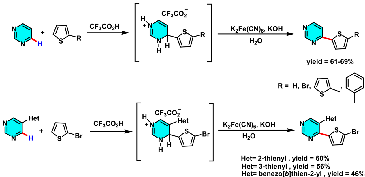
Scheme 66 Synthesis of 5-bromo-4-(hetero)arylpyrimidine derivatives via nucleophilic substitution of hydrogen ( S_NH ) reactions.
