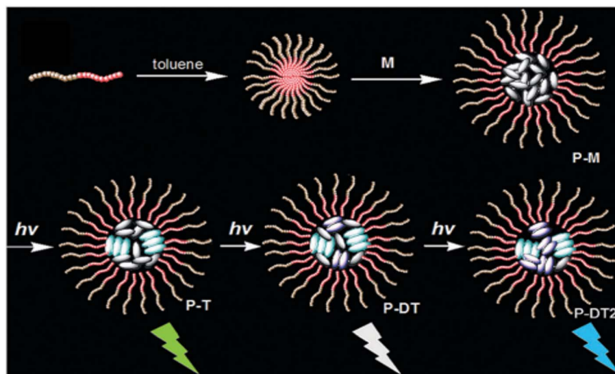
Fig. 106 Synthetic route of micellar ensemble P-M, with the encasement of the block copolymer P by diphenyl-diacetylene monomer M to form oligodiacetylene trimers (P-T) and dimers (P-DT and P-DT2). Reproduced from ref. 311, https://doi.org/10.1039/C5SC04253D , under the terms of the CC BY 4.0 license, https://creativecommons.org/licenses/by/4.0/ .
